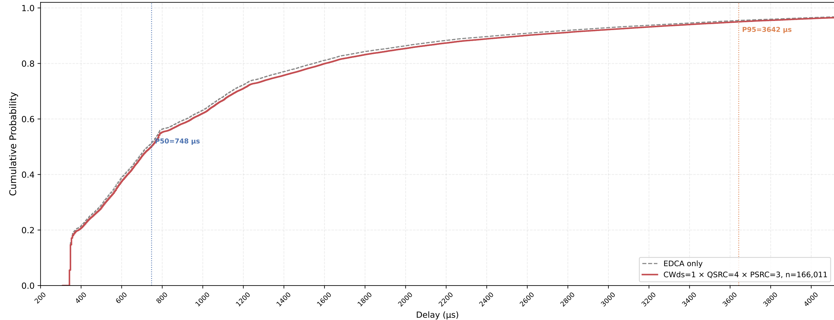
P-EDCA STA VO Delay CDF — CWds=1 × QSRC=4 × PSRC=3 nSta=30, nPedca=30, 0.5Mbps, avg of 10 runs
