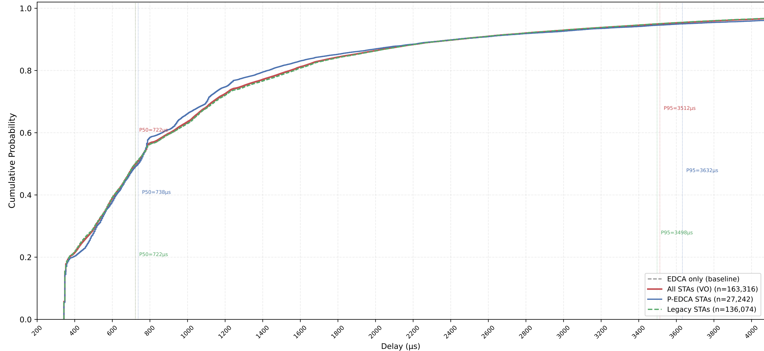
VO Delay CDF — P-EDCA / Legacy / All | CWds=1 × QSRC=5 × PSRC=1 nSta=30, nPedca=5/30, 0.5Mbps, avg of 10 runs
