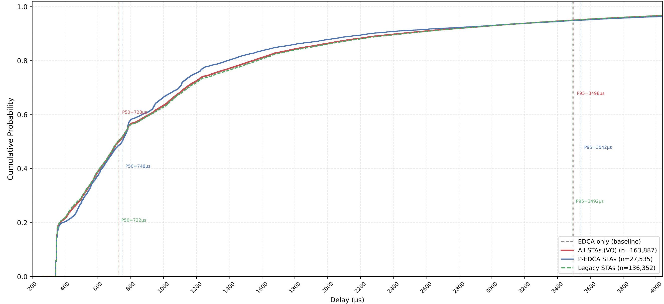
VO Delay CDF — P-EDCA / Legacy / All | CWds=1 × QSRC=5 × PSRC=2 nSta=30, nPedca=5/30, 0.5Mbps, avg of 10 runs
