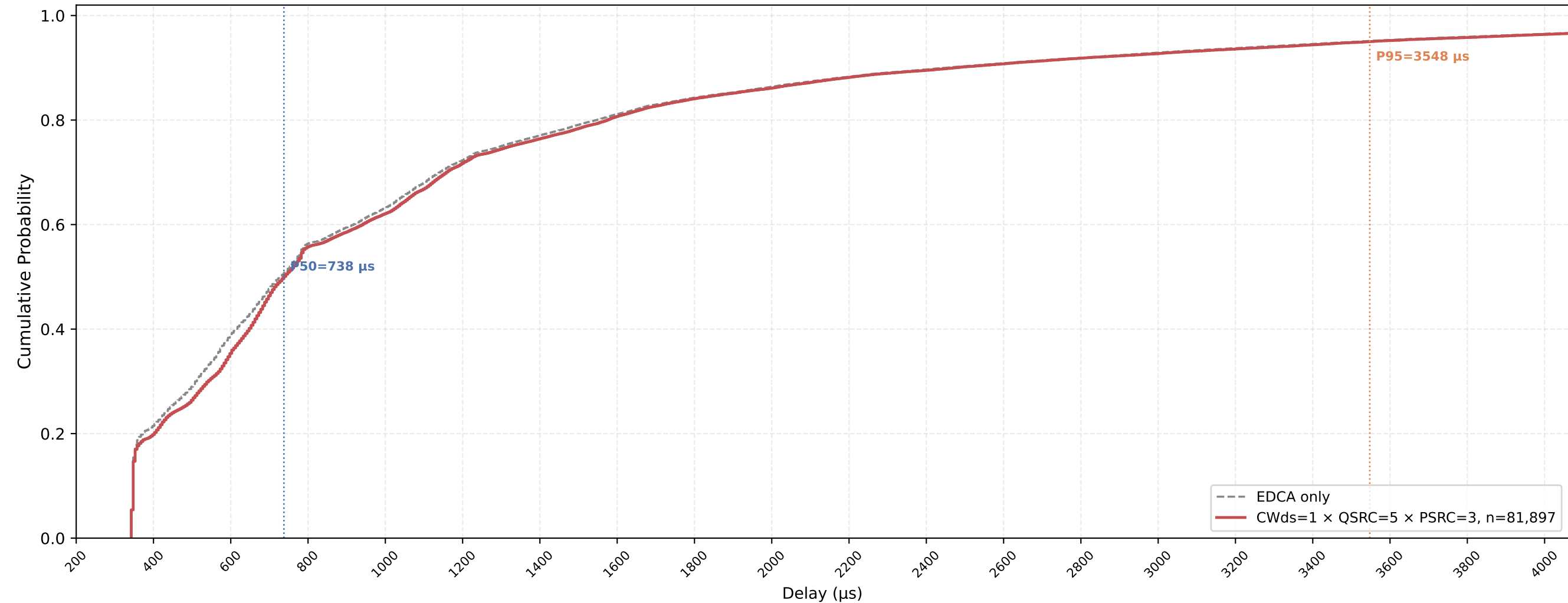
Legacy STA VO Delay CDF — CWds=1 × QSRC=5 × PSRC=3 nSta=30, nPedca=15, 0.5Mbps, avg of 10 runs
