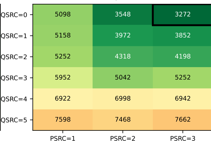
P-EDCA STA VO Delay — P95 Dual-DS (2x DS-CTS) (nSta=30, 1Mbps, black box = best in panel) colour scale 3272-10012 shared across mono-DS & dual-DS — panels are directly comparable
