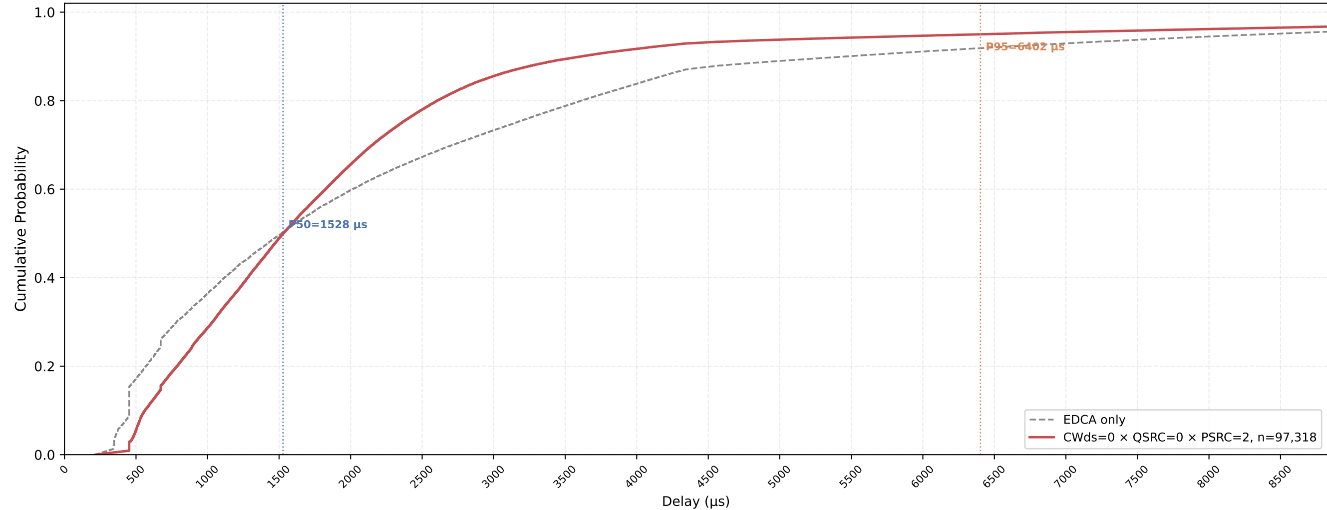
P-EDCA STA VO Delay CDF — CWds=0 × QSRC=0 × PSRC=2 nSta=30, nPedca=15, 1Mbps, avg of 10 runs
