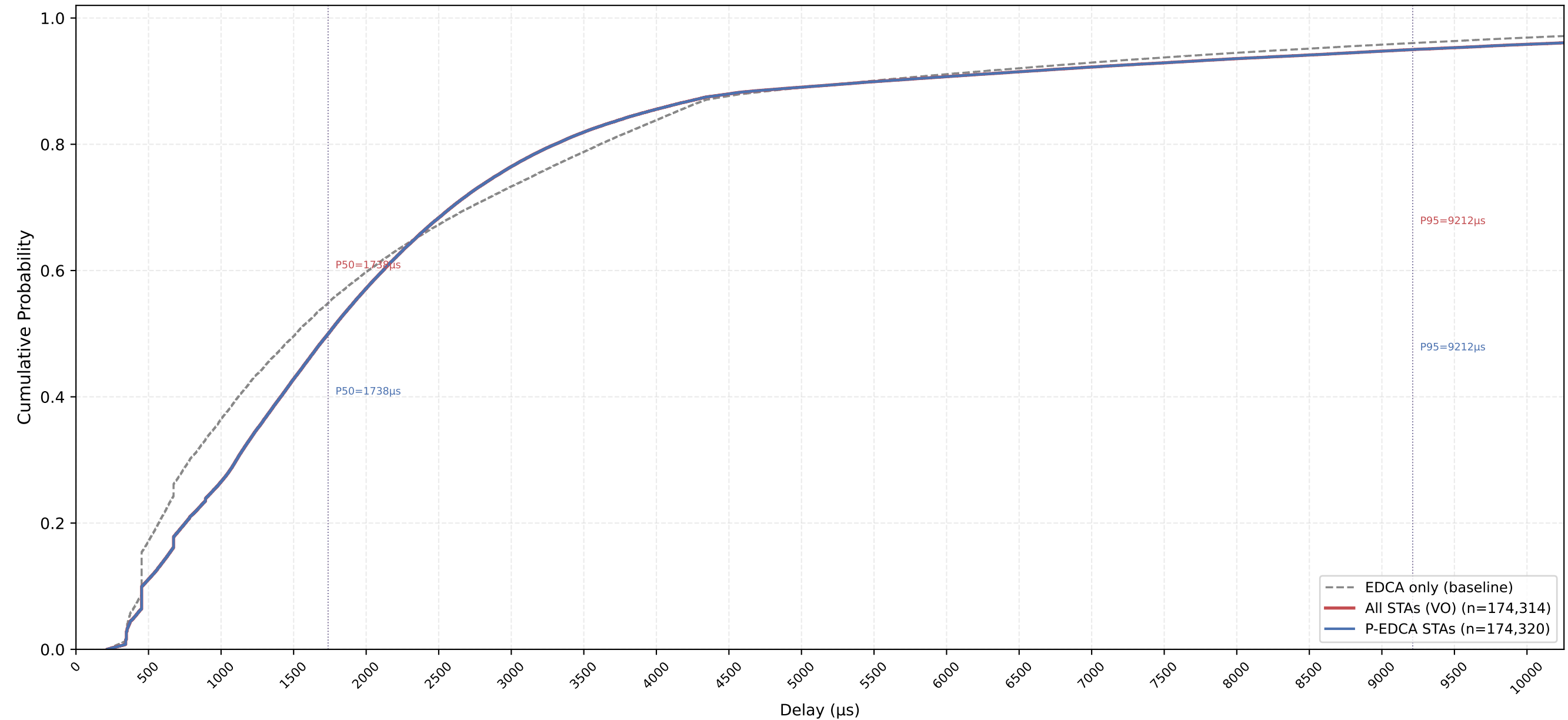
VO Delay CDF — P-EDCA / Legacy / All | CWds=0 × QSRC=1 × PSRC=1 nSta=30, nPedca=30/30, 1Mbps, avg of 10 runs
