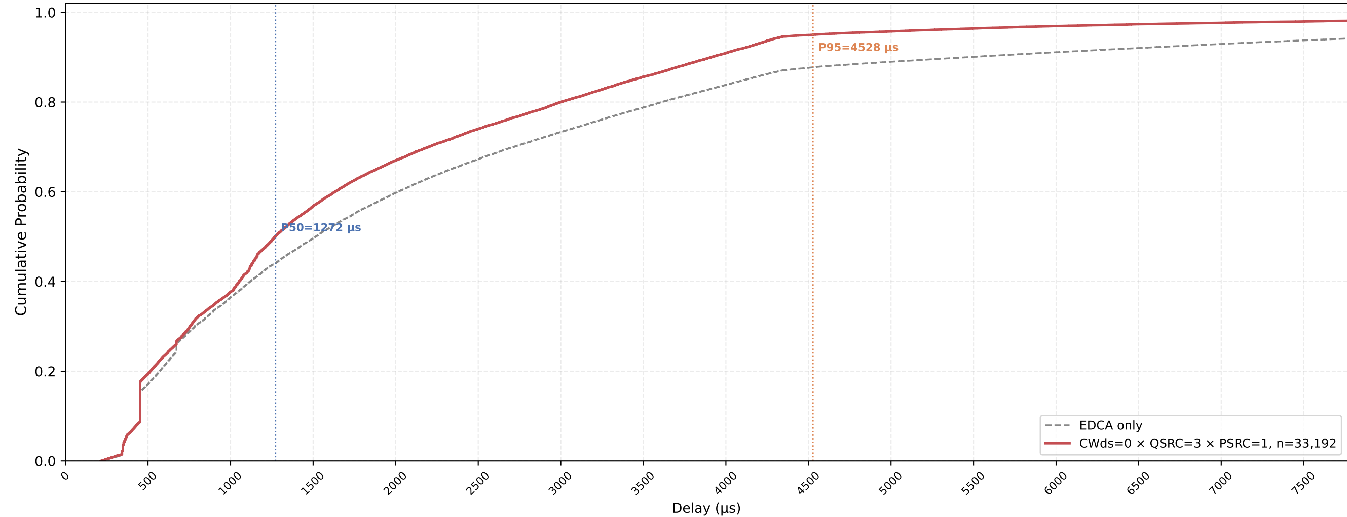
P-EDCA STA VO Delay CDF — CWds=0 × QSRC=3 × PSRC=1 nSta=30, nPedca=5, 1Mbps, avg of 10 runs
