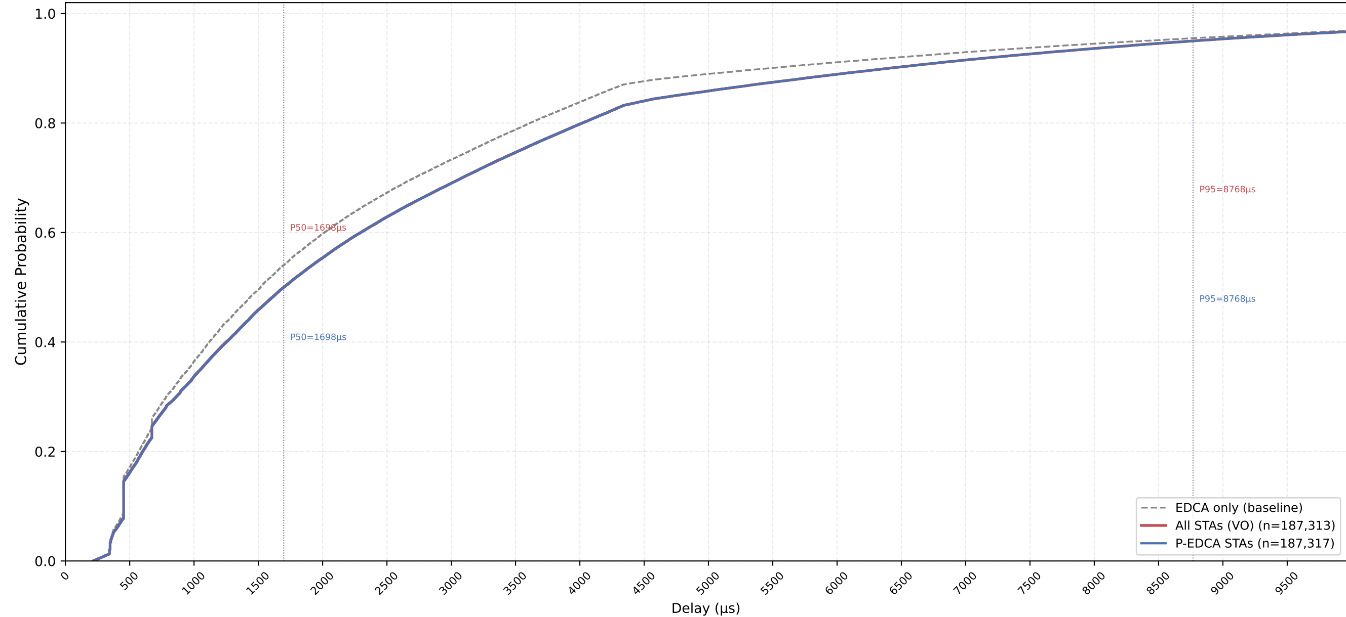
VO Delay CDF — P-EDCA / Legacy / All | CWds=0 × QSRC=5 × PSRC=2 nSta=30, nPedca=30/30, 1Mbps, avg of 10 runs
