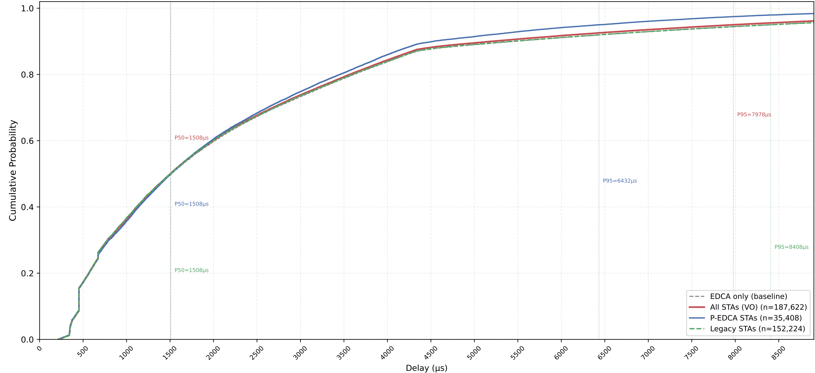
VO Delay CDF — P-EDCA / Legacy / All | CWds=0 × QSRC=5 × PSRC=3 nSta=30, nPedca=5/30, 1Mbps, avg of 10 runs
