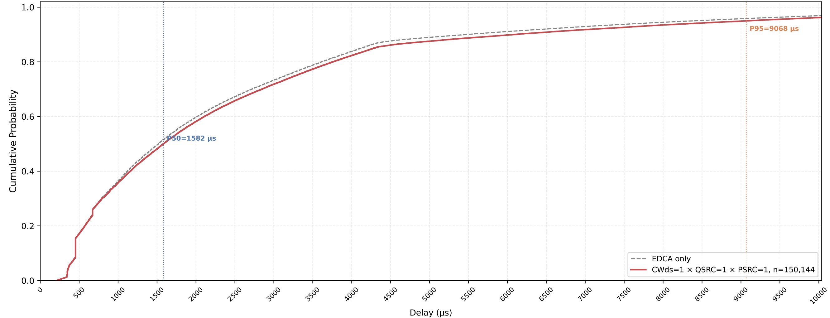
Legacy STA VO Delay CDF — CWds=1 × QSRC=1 × PSRC=1 nSta=30, nPedca=5, 1Mbps, avg of 10 runs
