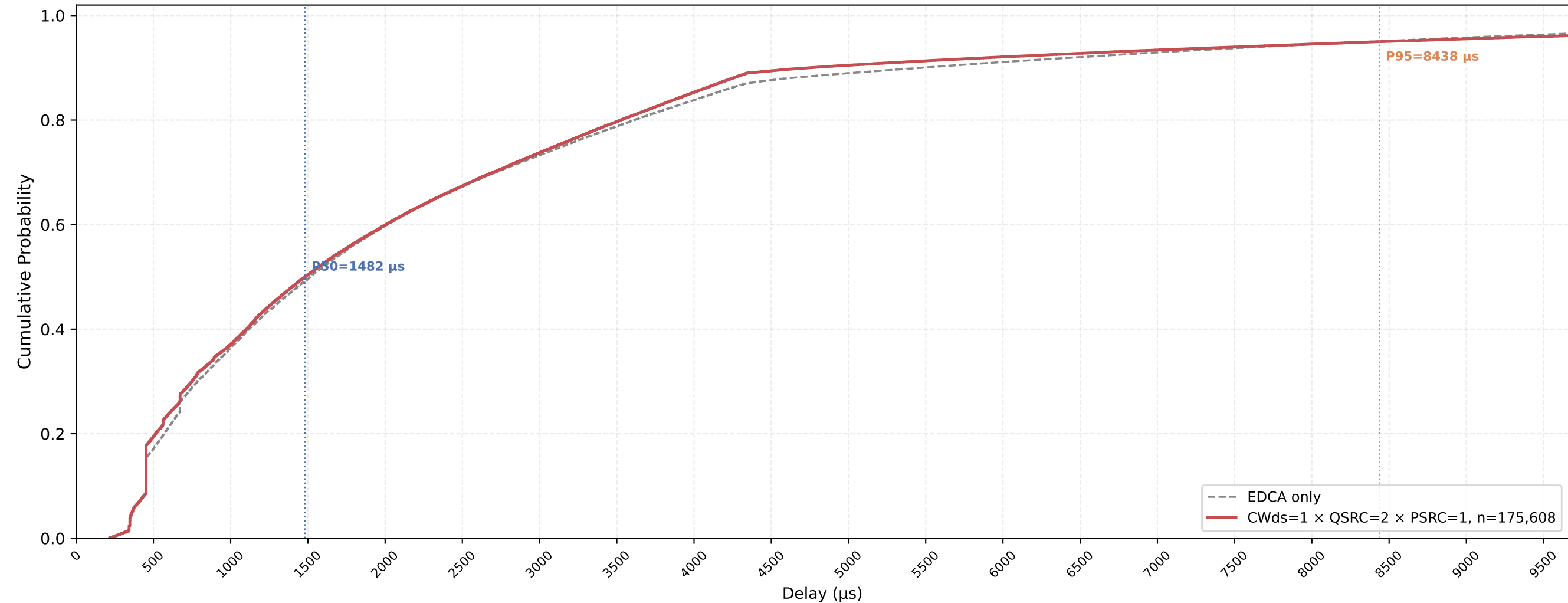
P-EDCA STA VO Delay CDF — CWds=1 × QSRC=2 × PSRC=1 nSta=30, nPedca=30, 1Mbps, avg of 10 runs
