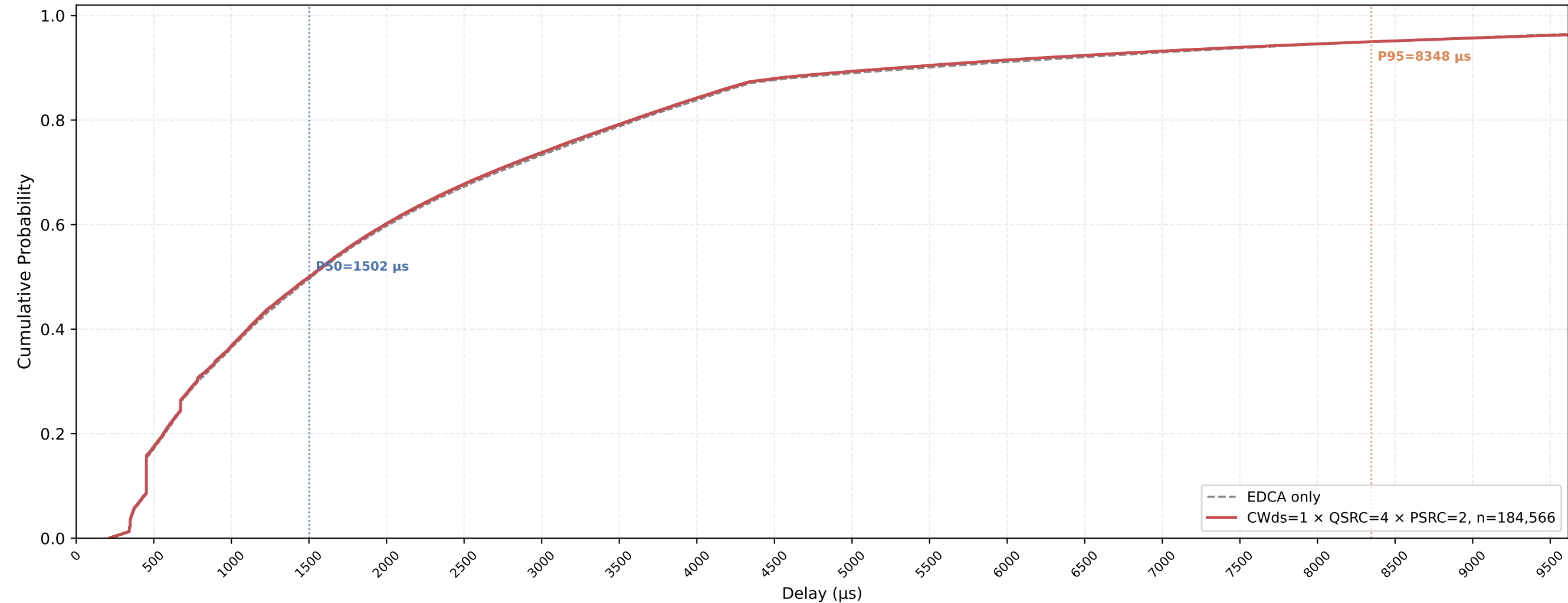
VO (all STAs) Delay CDF — CWds=1 × QSRC=4 × PSRC=2 nSta=30, nPedca=15, 1Mbps, avg of 10 runs
