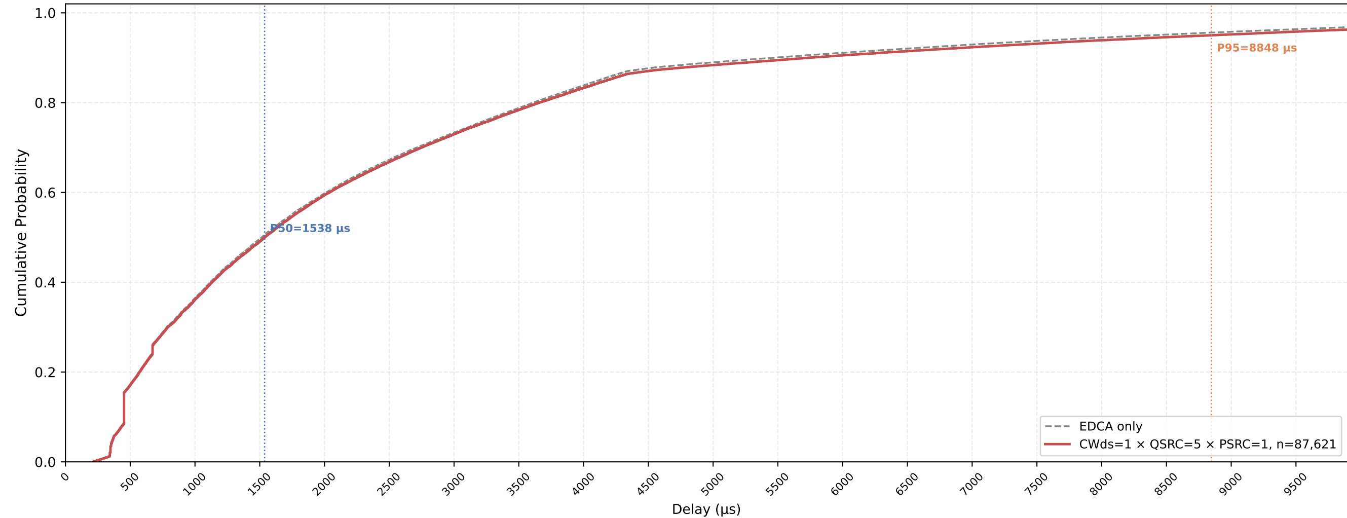
Legacy STA VO Delay CDF — CWds=1 × QSRC=5 × PSRC=1 nSta=30, nPedca=15, 1Mbps, avg of 10 runs
