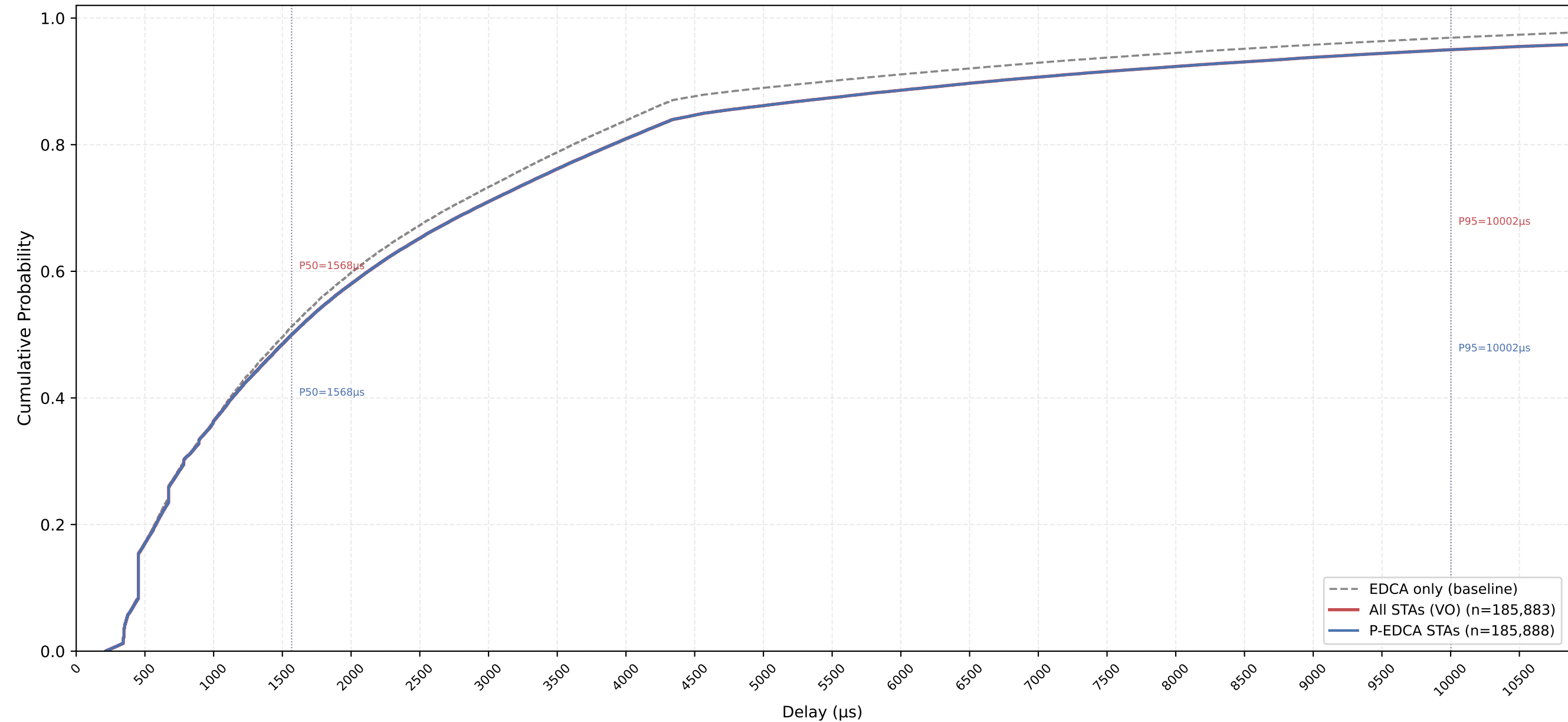
VO Delay CDF — P-EDCA / Legacy / All | CWds=1 × QSRC=5 × PSRC=3 nSta=30, nPedca=30/30, 1Mbps, avg of 10 runs
