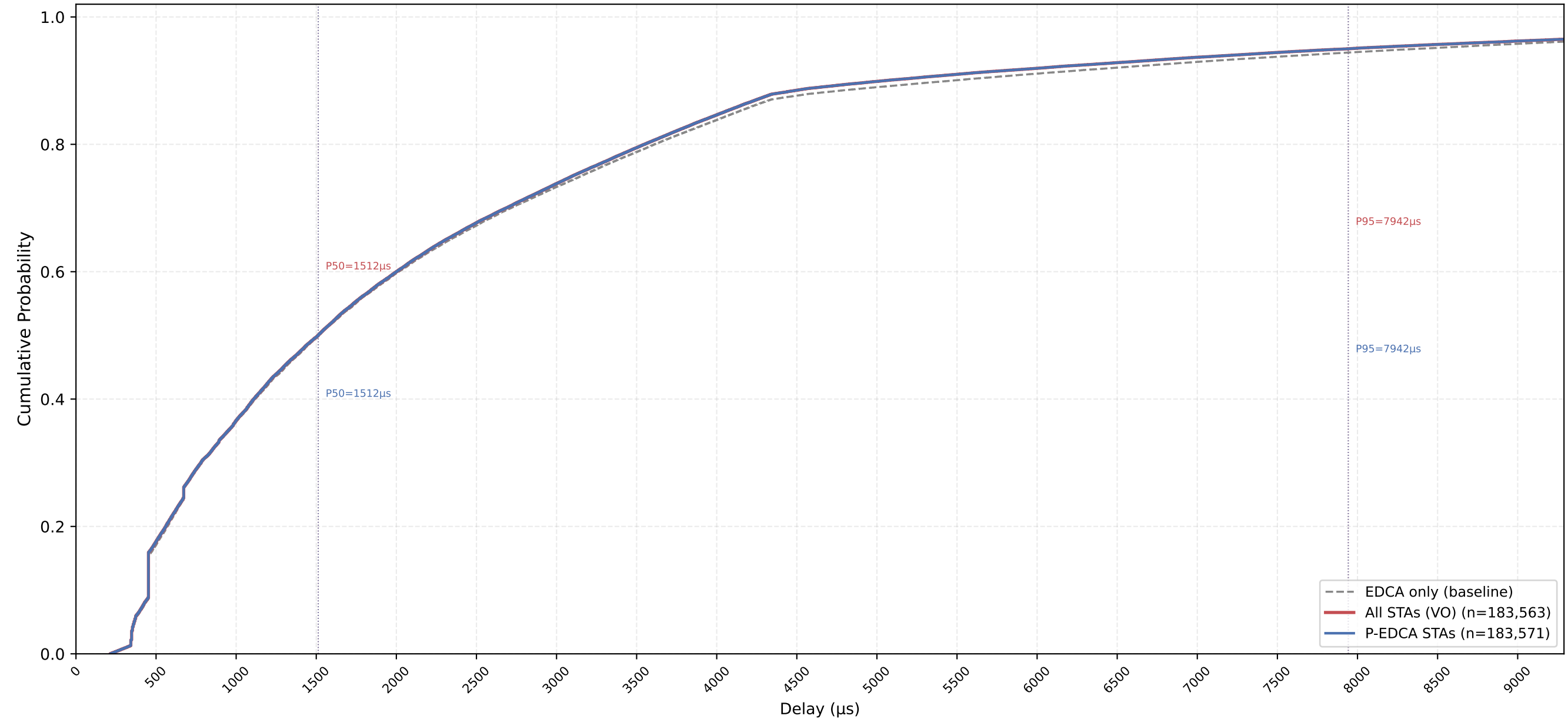
VO Delay CDF — P-EDCA / Legacy / All | CWds=0 × QSRC=4 × PSRC=2 nSta=30, nPedca=30/30, 1Mbps, avg of 10 runs
