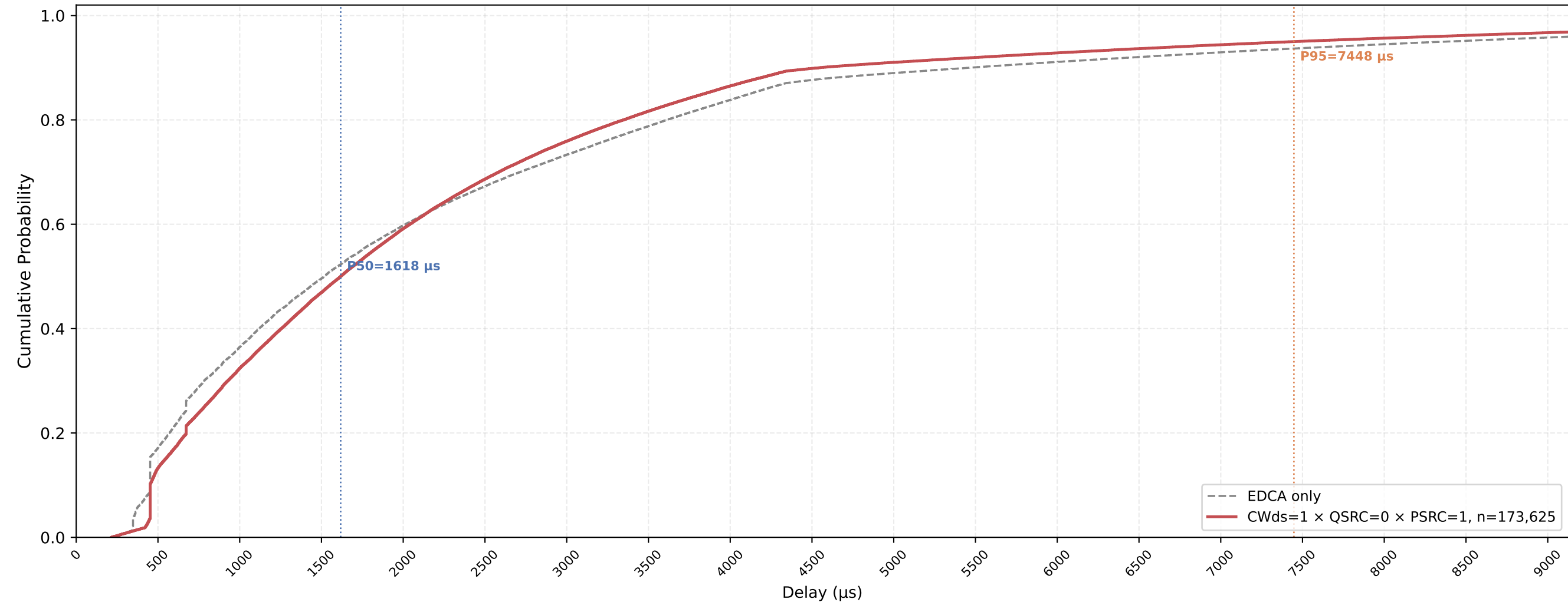
P-EDCA STA VO Delay CDF — CWds=1 × QSRC=0 × PSRC=1 nSta=30, nPedca=30, 1Mbps, avg of 10 runs
