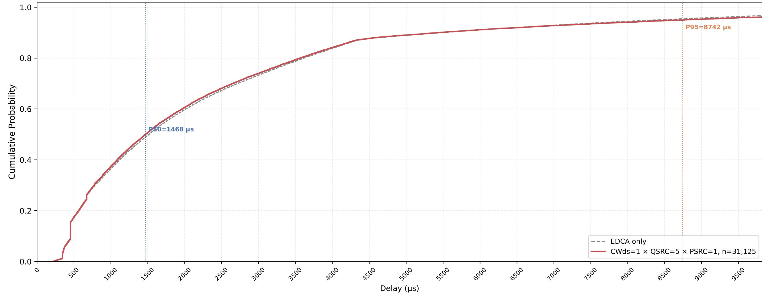
P-EDCA STA VO Delay CDF — CWds=1 × QSRC=5 × PSRC=1 nSta=30, nPedca=5, 1Mbps, avg of 10 runs
