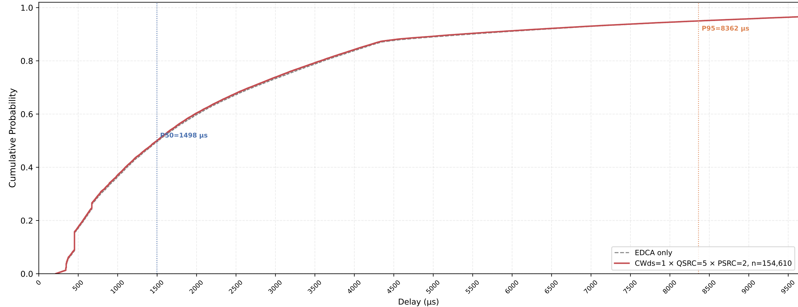
Legacy STA VO Delay CDF — CWds=1 × QSRC=5 × PSRC=2 nSta=30, nPedca=5, 1Mbps, avg of 10 runs
