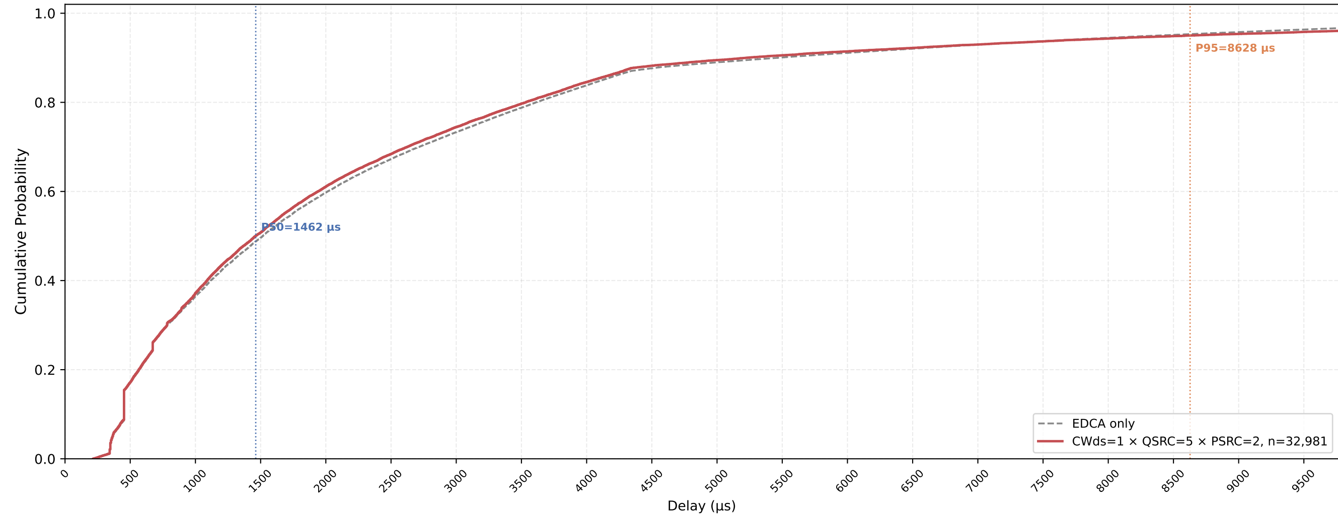
P-EDCA STA VO Delay CDF — CWds=1 × QSRC=5 × PSRC=2 nSta=30, nPedca=5, 1Mbps, avg of 10 runs
