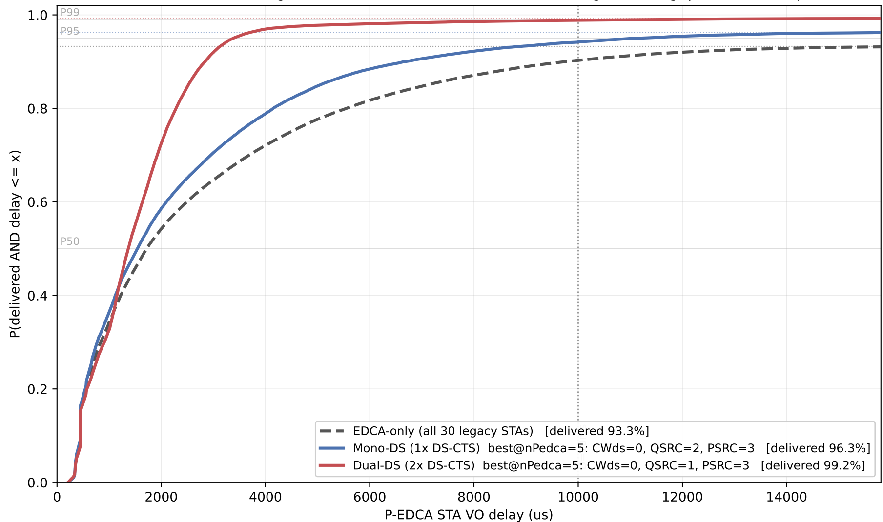
P-EDCA STA Delay CDF at Best Parameters (nPedca=5/30, nSta=30, 1Mbps) curves saturate at each configuration's delivered fraction (dotted ceilings) — the gap below 1.0 is packet loss
