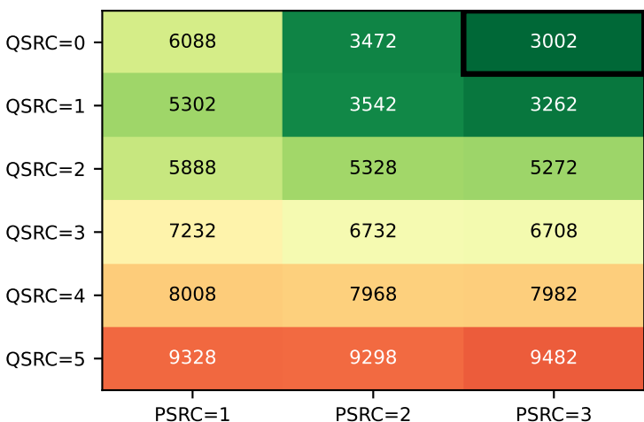
P-EDCA STA VO Delay — P95 Dual-DS (2x DS-CTS) (nSta=30, 1Mbps, black box = best in panel) colour scale 3002-10862 shared across mono-DS & dual-DS — panels are directly comparable
