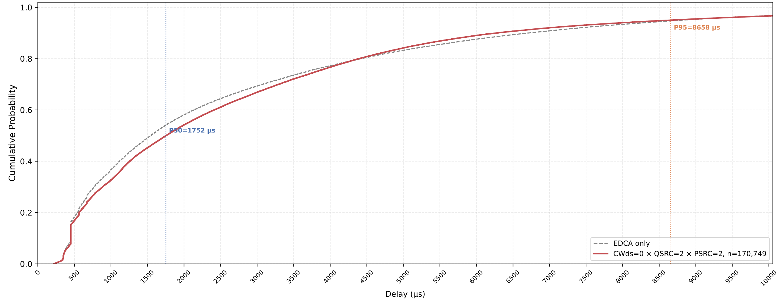
VO (all STAs) Delay CDF — CWds=0 × QSRC=2 × PSRC=2 nSta=30, nPedca=15, 1Mbps, avg of 10 runs
