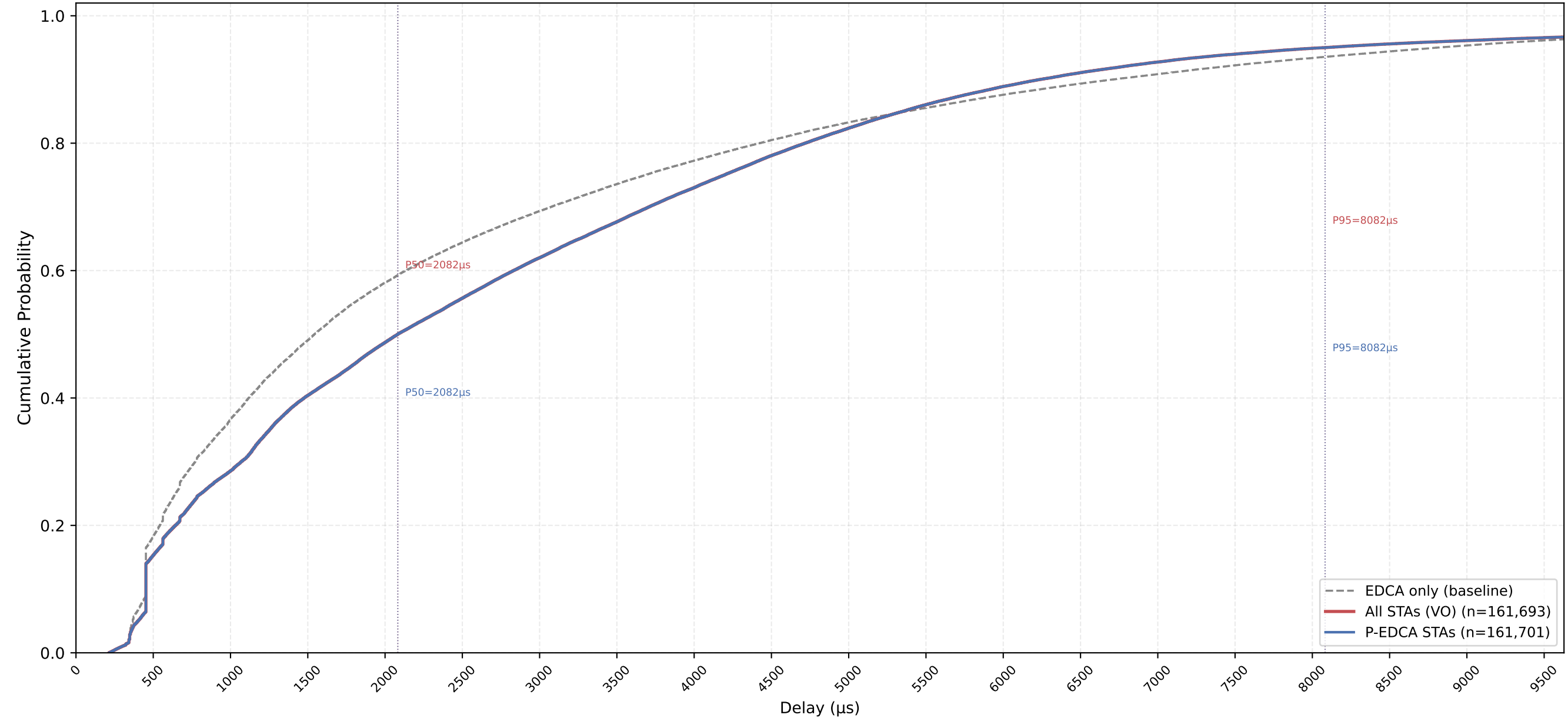
VO Delay CDF — P-EDCA / Legacy / All | CWds=0 × QSRC=2 × PSRC=3 nSta=30, nPedca=30/30, 1Mbps, avg of 10 runs
