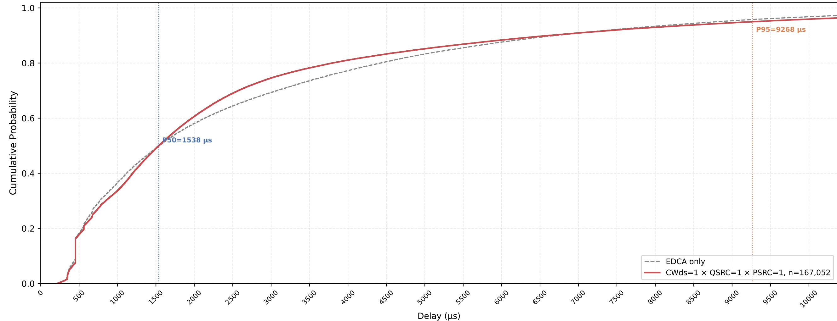
P-EDCA STA VO Delay CDF — CWds=1 × QSRC=1 × PSRC=1 nSta=30, nPedca=30, 1Mbps, avg of 10 runs
