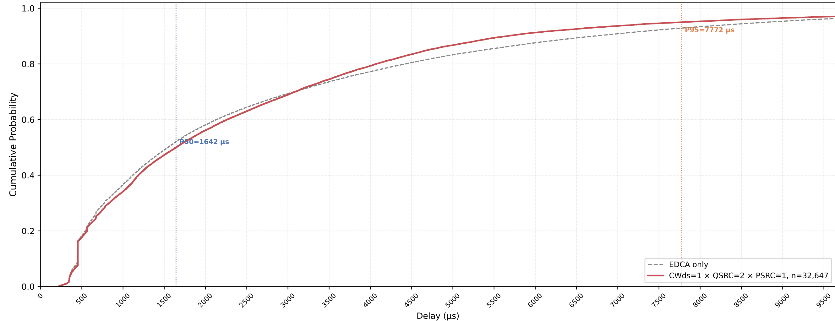
P-EDCA STA VO Delay CDF — CWds=1 × QSRC=2 × PSRC=1 nSta=30, nPedca=5, 1Mbps, avg of 10 runs
