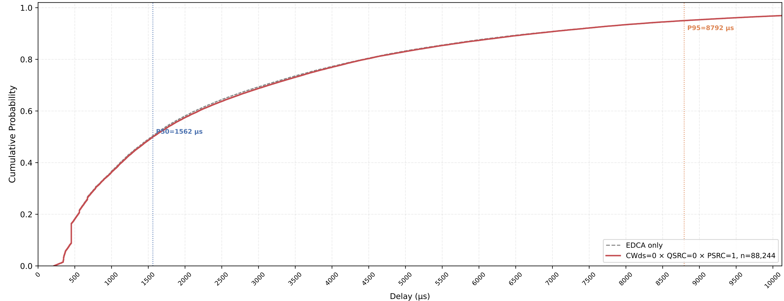
Legacy STA VO Delay CDF — CWds=0 × QSRC=0 × PSRC=1 nSta=30, nPedca=15, 1Mbps, avg of 10 runs
