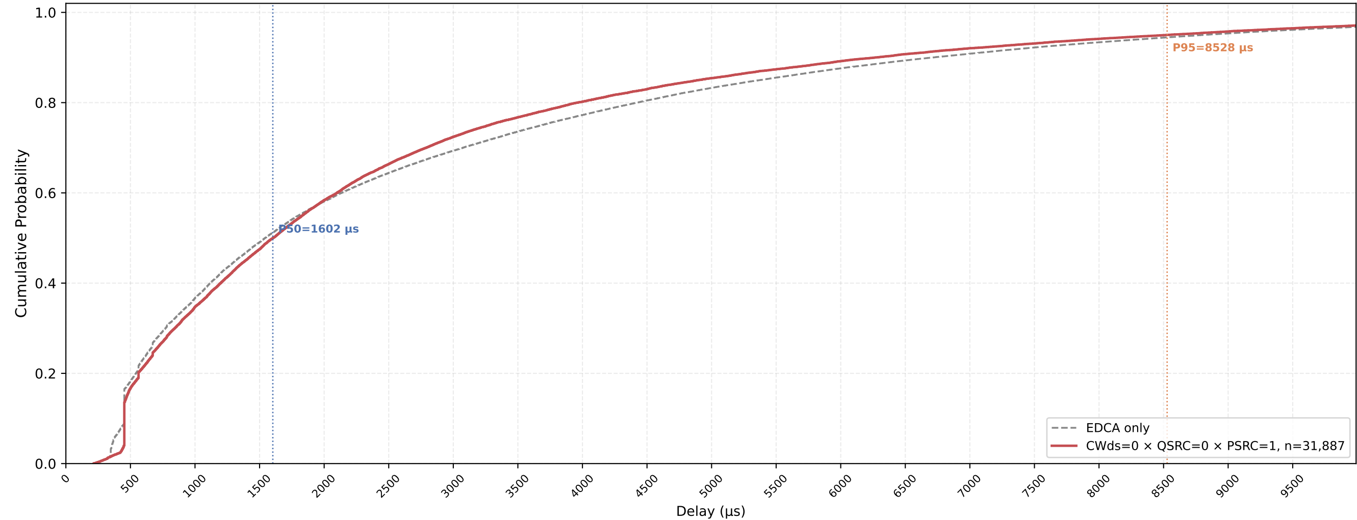
P-EDCA STA VO Delay CDF — CWds=0 × QSRC=0 × PSRC=1 nSta=30, nPedca=5, 1Mbps, avg of 10 runs
