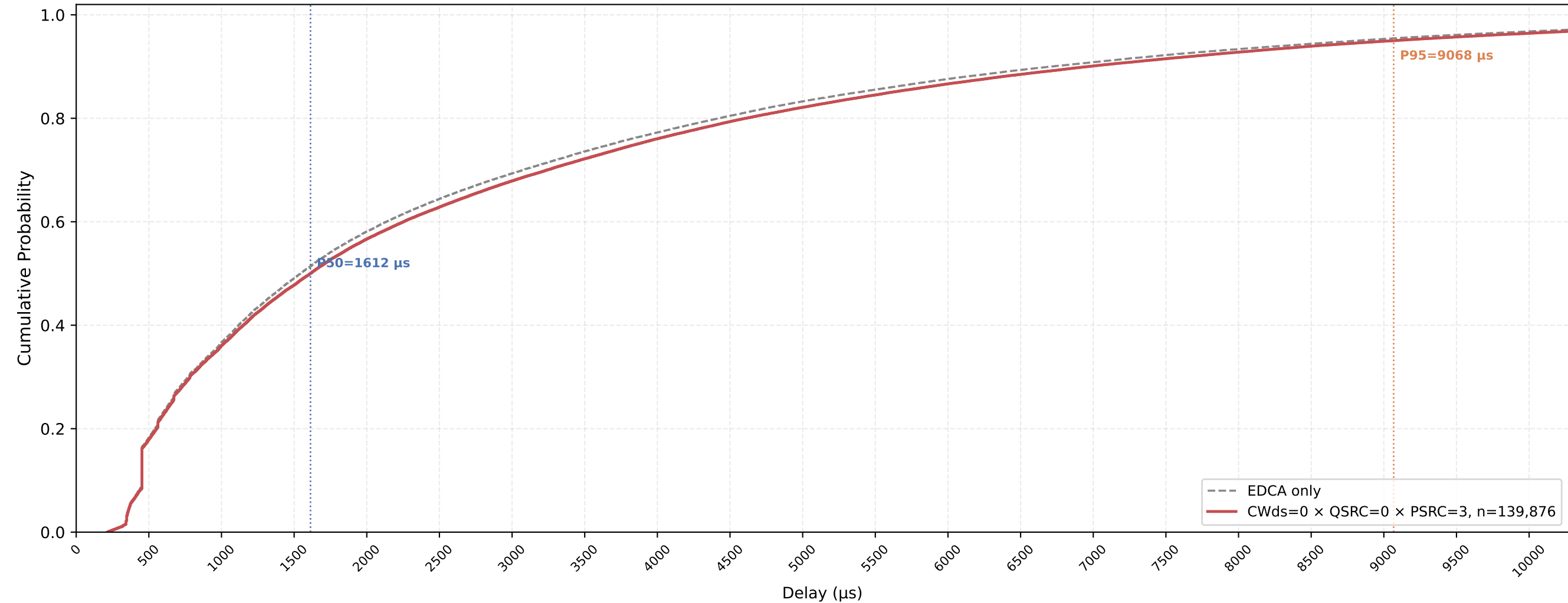
Legacy STA VO Delay CDF — CWds=0 × QSRC=0 × PSRC=3 nSta=30, nPedca=5, 1Mbps, avg of 10 runs
