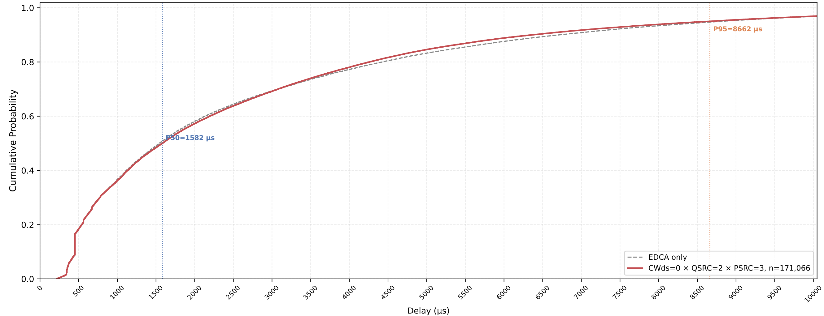
VO (all STAs) Delay CDF — CWds=0 × QSRC=2 × PSRC=3 nSta=30, nPedca=30, 1Mbps, avg of 10 runs
