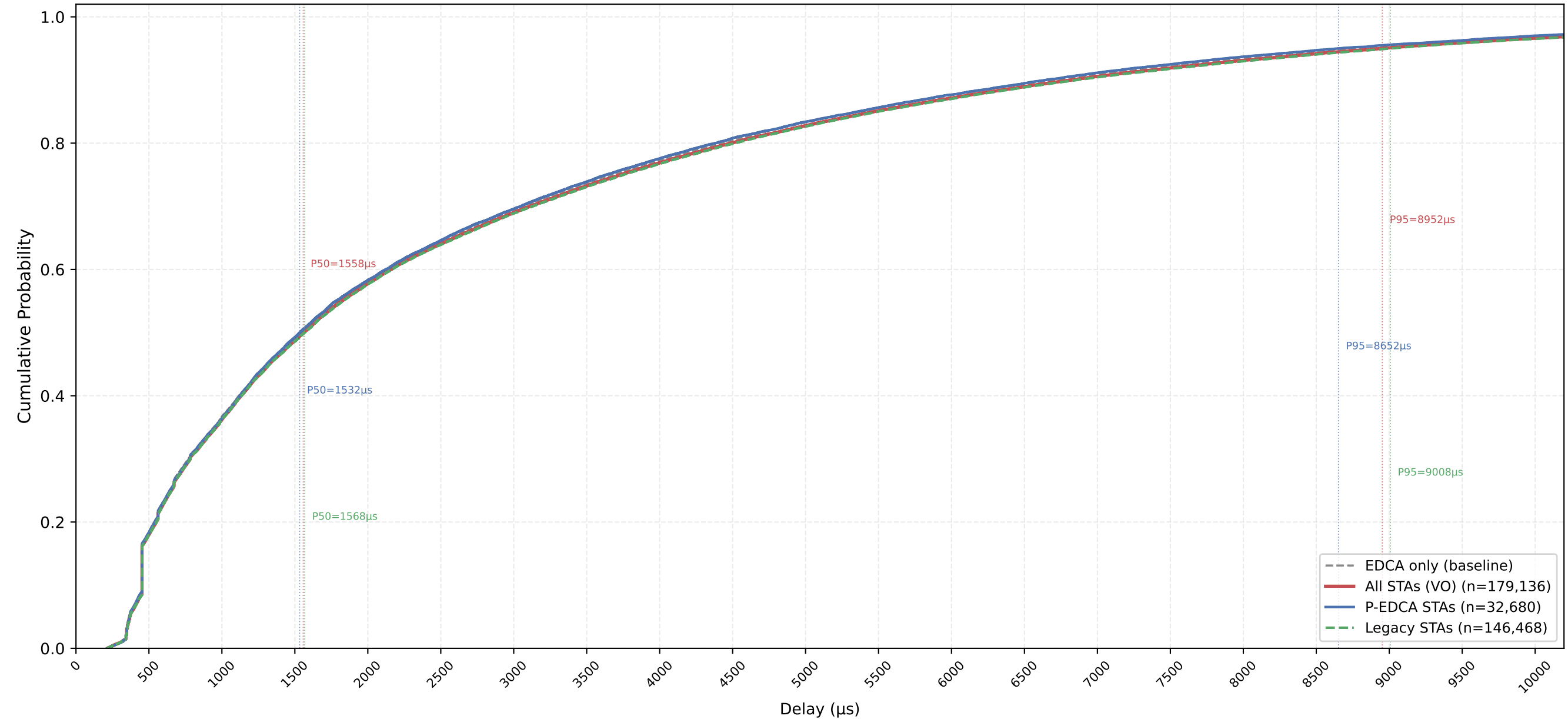
VO Delay CDF — P-EDCA / Legacy / All | CWds=0 × QSRC=5 × PSRC=2 nSta=30, nPedca=5/30, 1Mbps, avg of 10 runs
