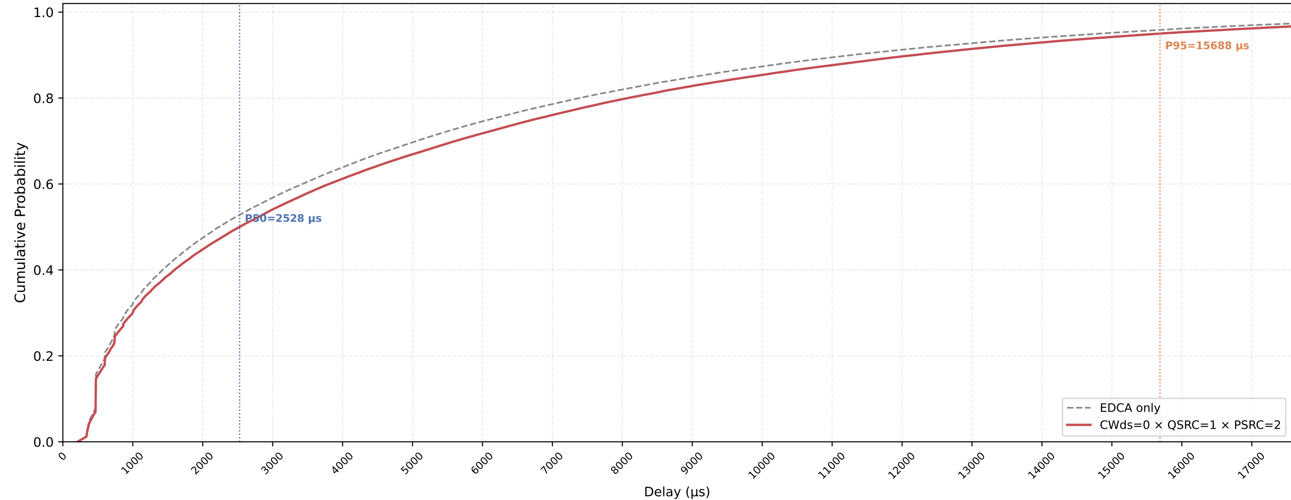
Legacy STA VO Delay CDF — CWds=0 × QSRC=1 × PSRC=2 nSta=30, nPedca=5, 1Mbps, avg of 10 runs
