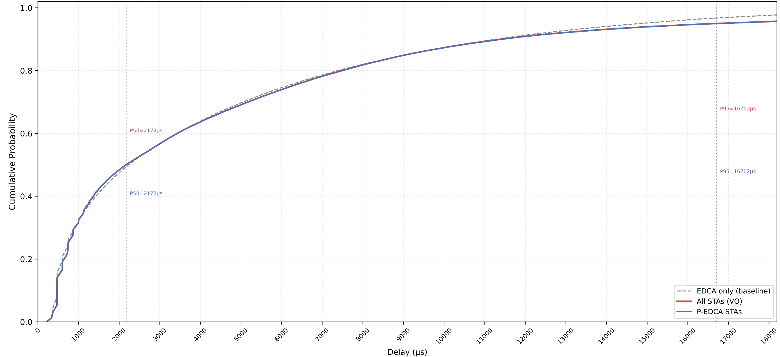
VO Delay CDF — P-EDCA / Legacy / All | CWds=0 × QSRC=3 × PSRC=3 nSta=30, nPedca=30/30, 1Mbps, avg of 10 runs
