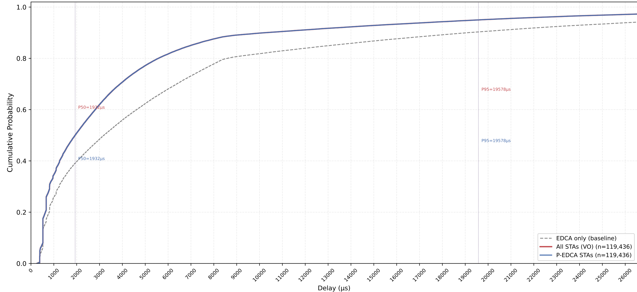
VO Delay CDF — P-EDCA / Legacy / All | CWds=0 × QSRC=1 × PSRC=2 nSta=30, nPedca=30/30, 1Mbps, avg of 10 runs
