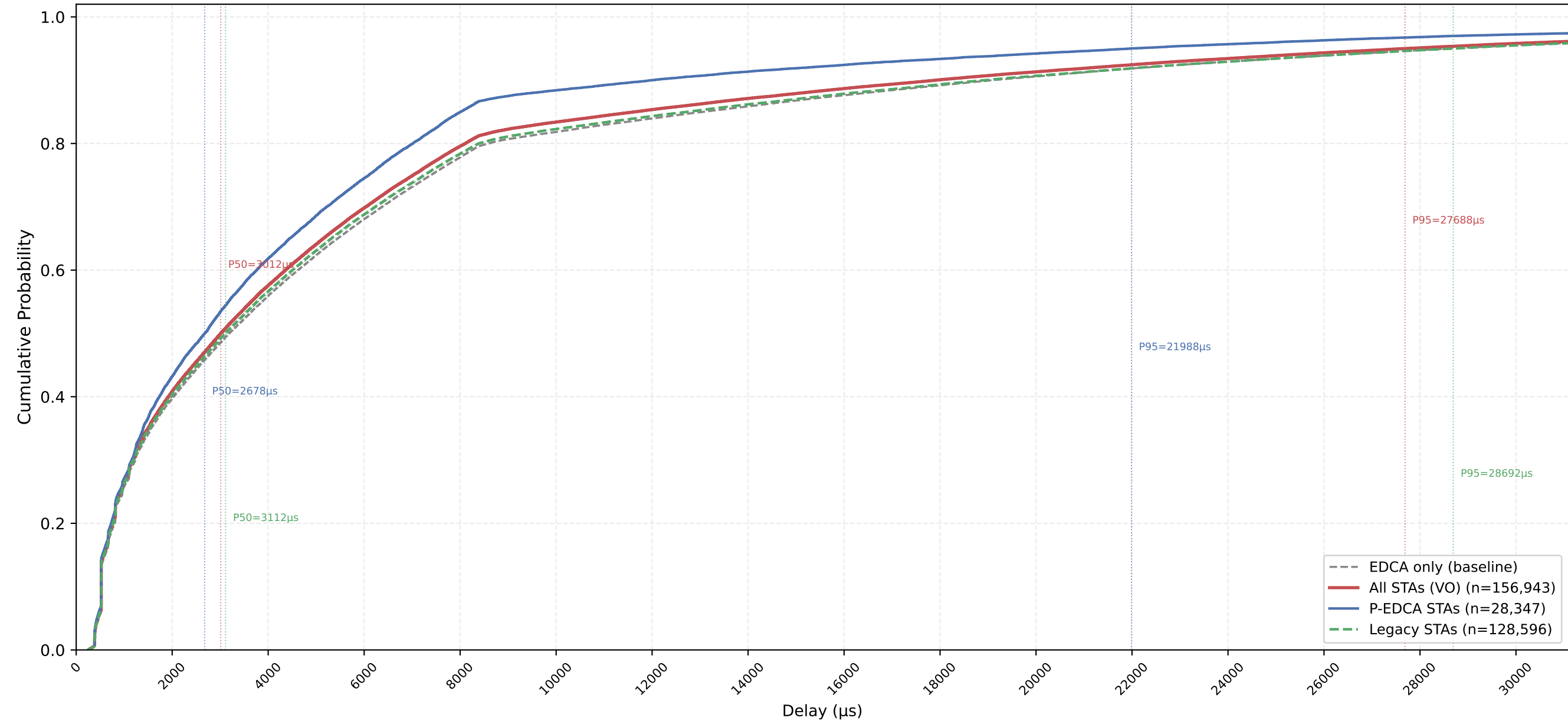
VO Delay CDF — P-EDCA / Legacy / All | CWds=0 × QSRC=3 × PSRC=1 nSta=30, nPedca=5/30, 1Mbps, avg of 10 runs
