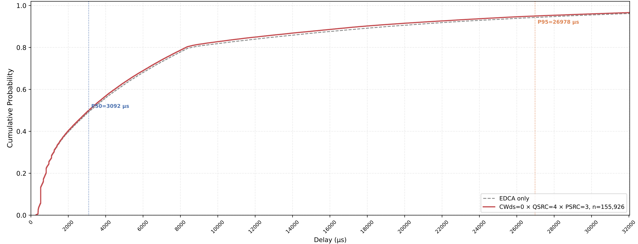
VO (all STAs) Delay CDF — CWds=0 × QSRC=4 × PSRC=3 nSta=30, nPedca=15, 1Mbps, avg of 10 runs
