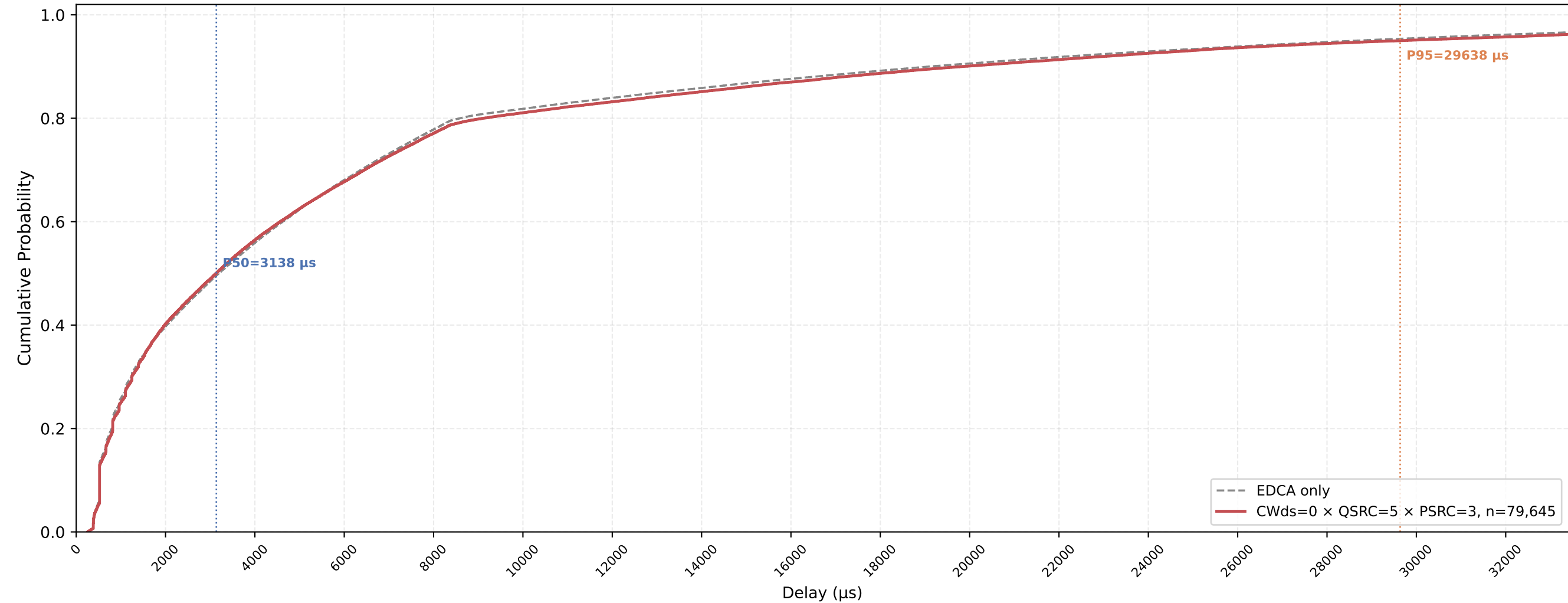
P-EDCA STA VO Delay CDF — CWds=0 × QSRC=5 × PSRC=3 nSta=30, nPedca=15, 1Mbps, avg of 10 runs
