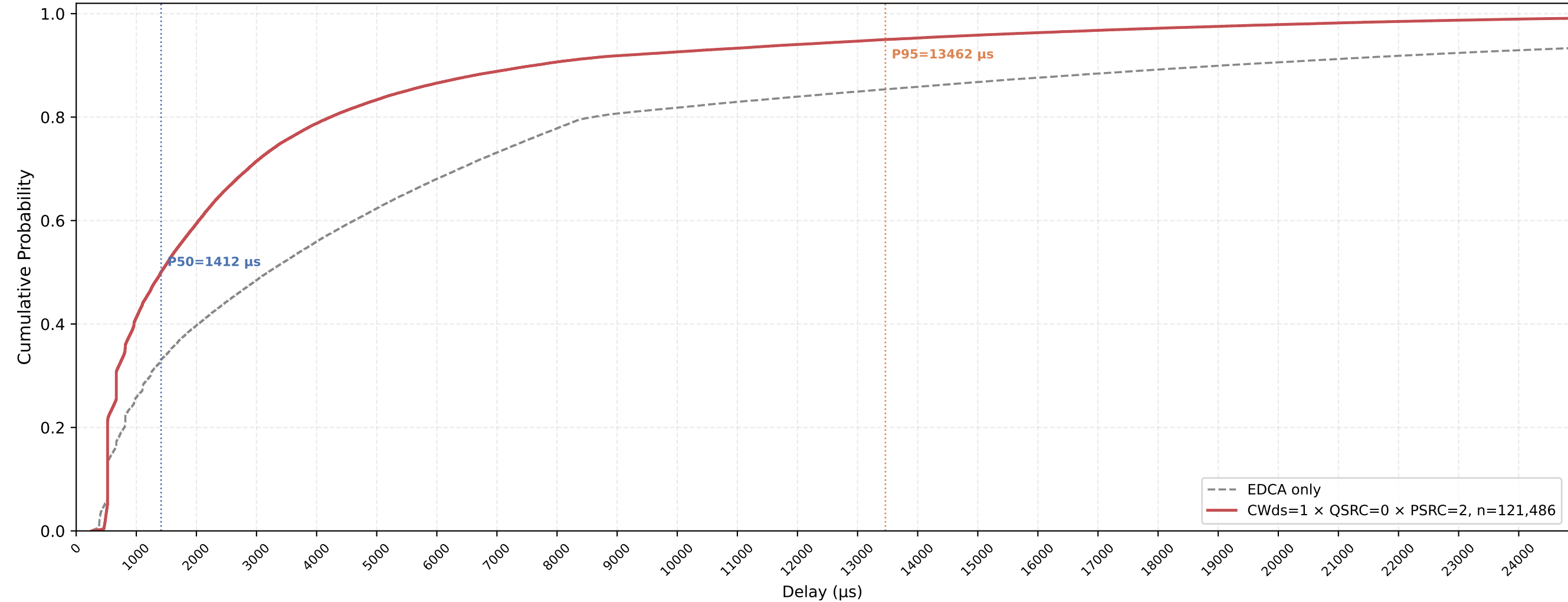
P-EDCA STA VO Delay CDF — CWds=1 × QSRC=0 × PSRC=2 nSta=30, nPedca=30, 1Mbps, avg of 10 runs
