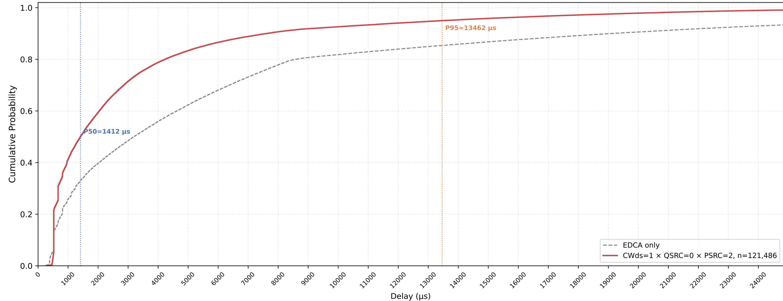
VO (all STAs) Delay CDF — CWds=1 × QSRC=0 × PSRC=2 nSta=30, nPedca=30, 1Mbps, avg of 10 runs
