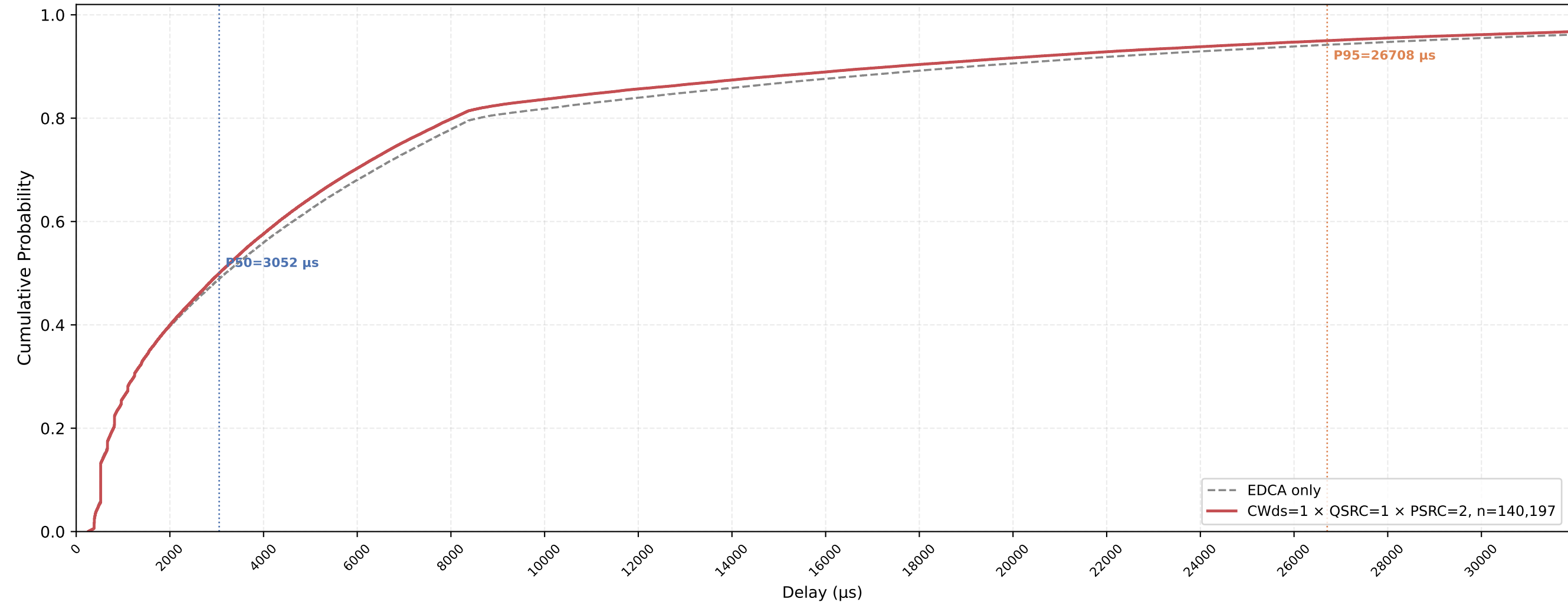
VO (all STAs) Delay CDF — CWds=1 × QSRC=1 × PSRC=2 nSta=30, nPedca=5, 1Mbps, avg of 10 runs
