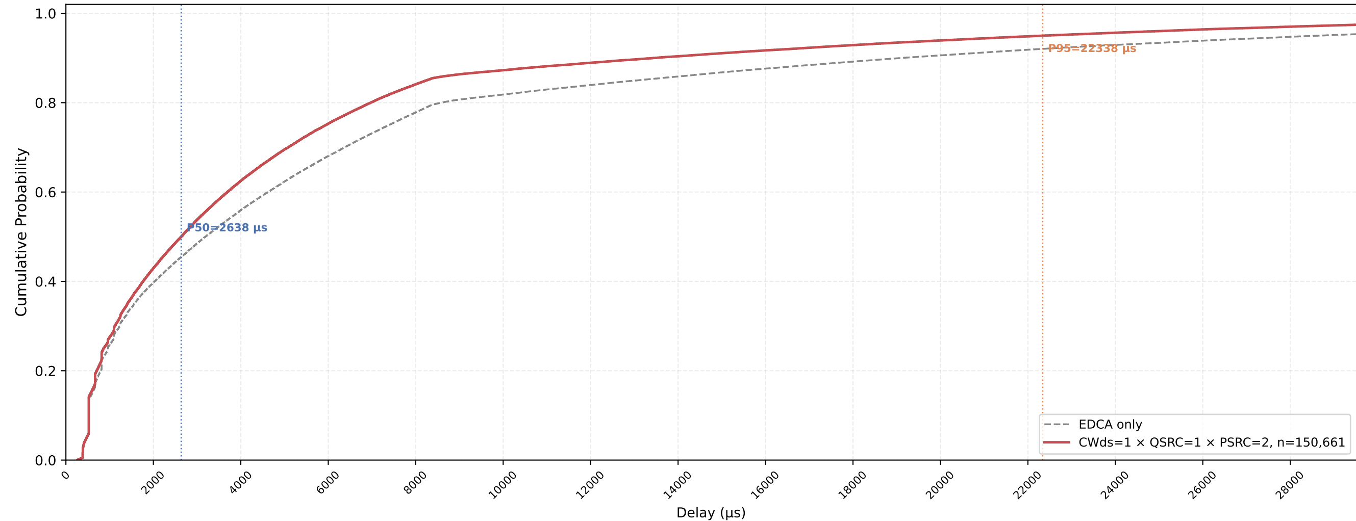
VO (all STAs) Delay CDF — CWds=1 × QSRC=1 × PSRC=2 nSta=30, nPedca=15, 1Mbps, avg of 10 runs
