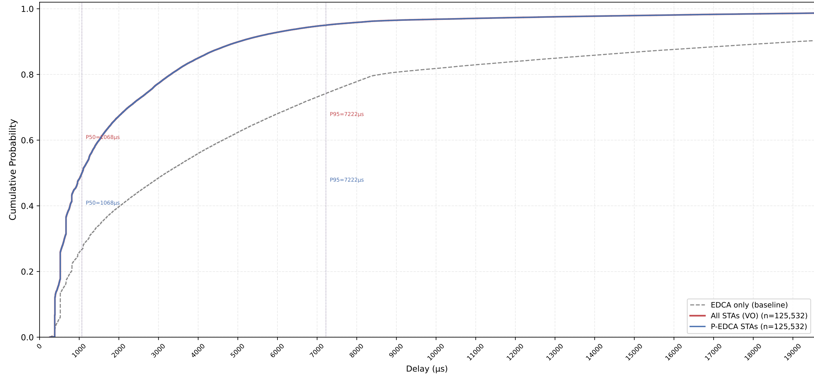
VO Delay CDF — P-EDCA / Legacy / All | CWds=1 × QSRC=1 × PSRC=3 nSta=30, nPedca=30/30, 1Mbps, avg of 10 runs
