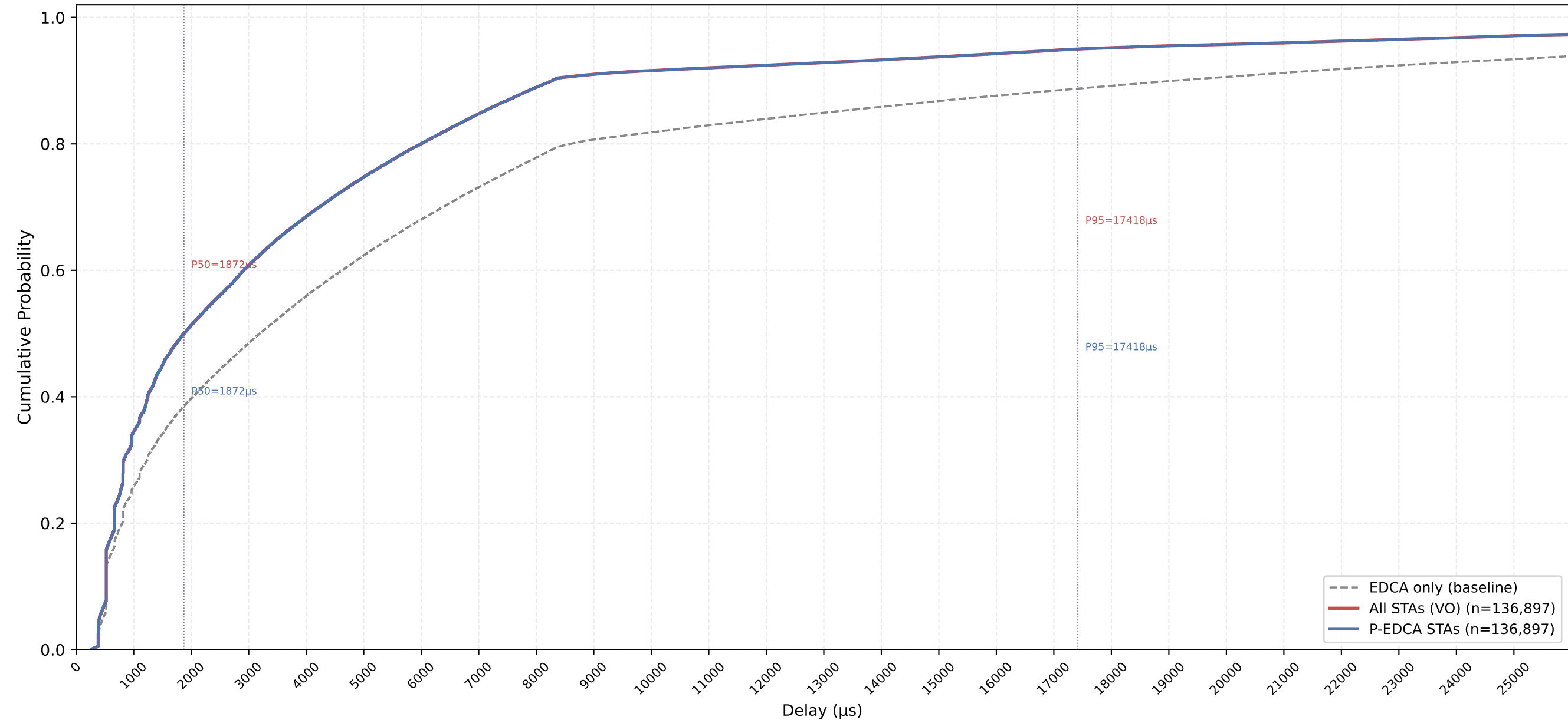
VO Delay CDF — P-EDCA / Legacy / All | CWds=1 × QSRC=2 × PSRC=3 nSta=30, nPedca=30/30, 1Mbps, avg of 10 runs
