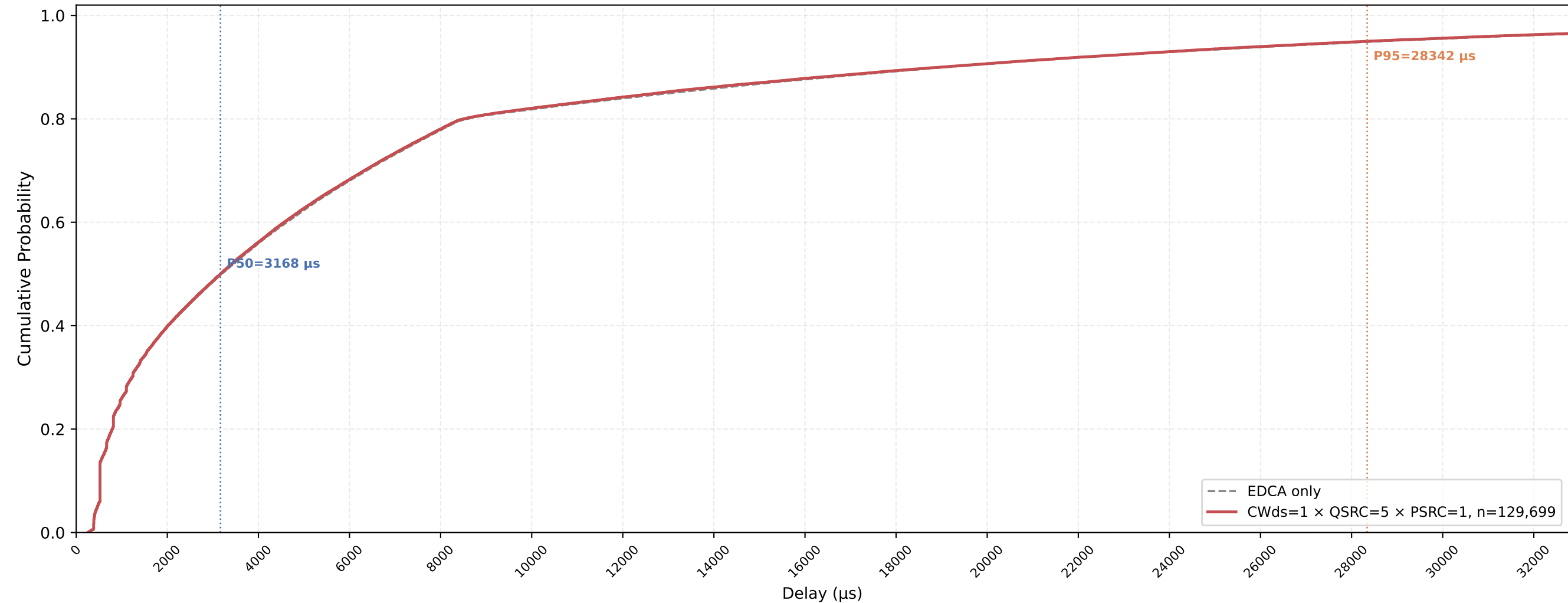
Legacy STA VO Delay CDF — CWds=1 × QSRC=5 × PSRC=1 nSta=30, nPedca=5, 1Mbps, avg of 10 runs
