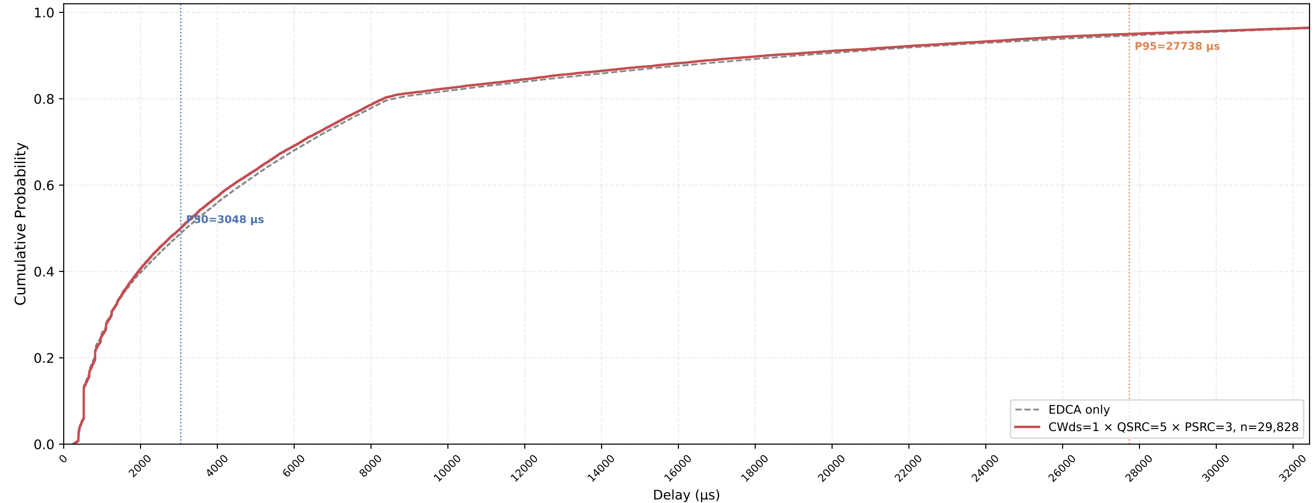
P-EDCA STA VO Delay CDF — CWds=1 × QSRC=5 × PSRC=3 nSta=30, nPedca=5, 1Mbps, avg of 10 runs
