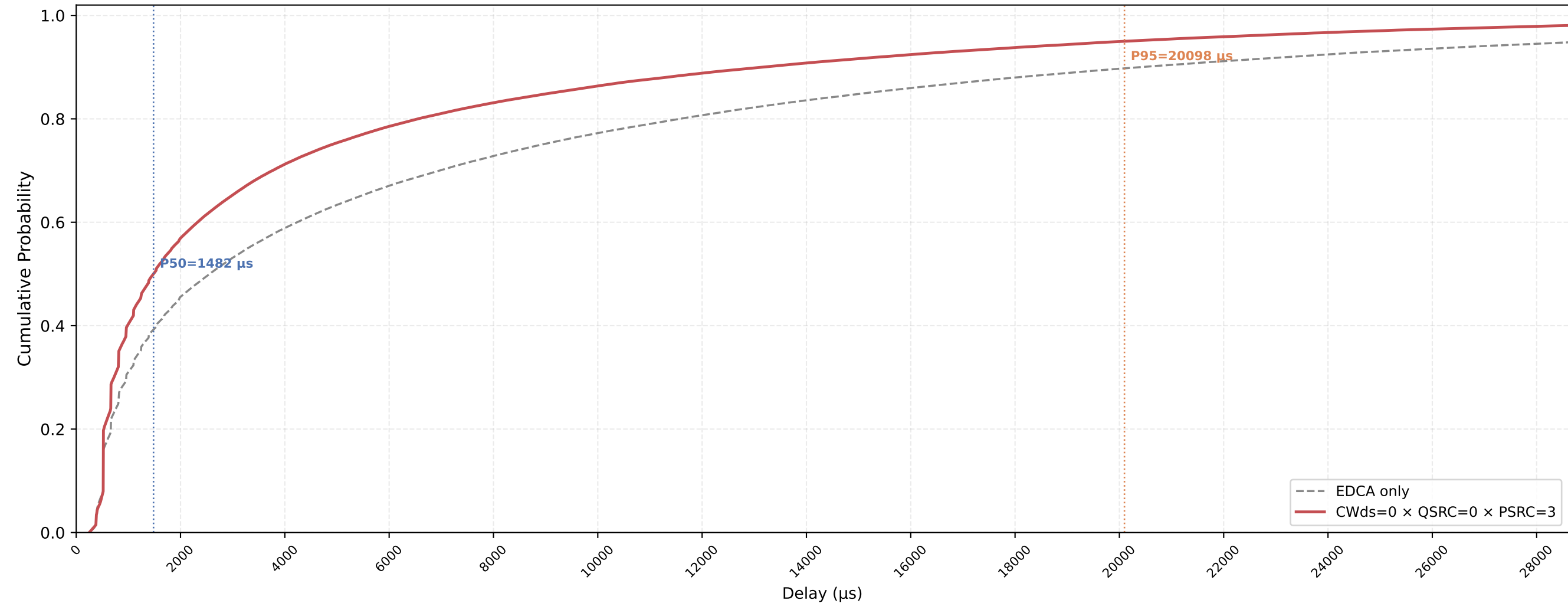
VO (all STAs) Delay CDF — CWds=0 × QSRC=0 × PSRC=3 nSta=30, nPedca=15, 1Mbps, avg of 10 runs
