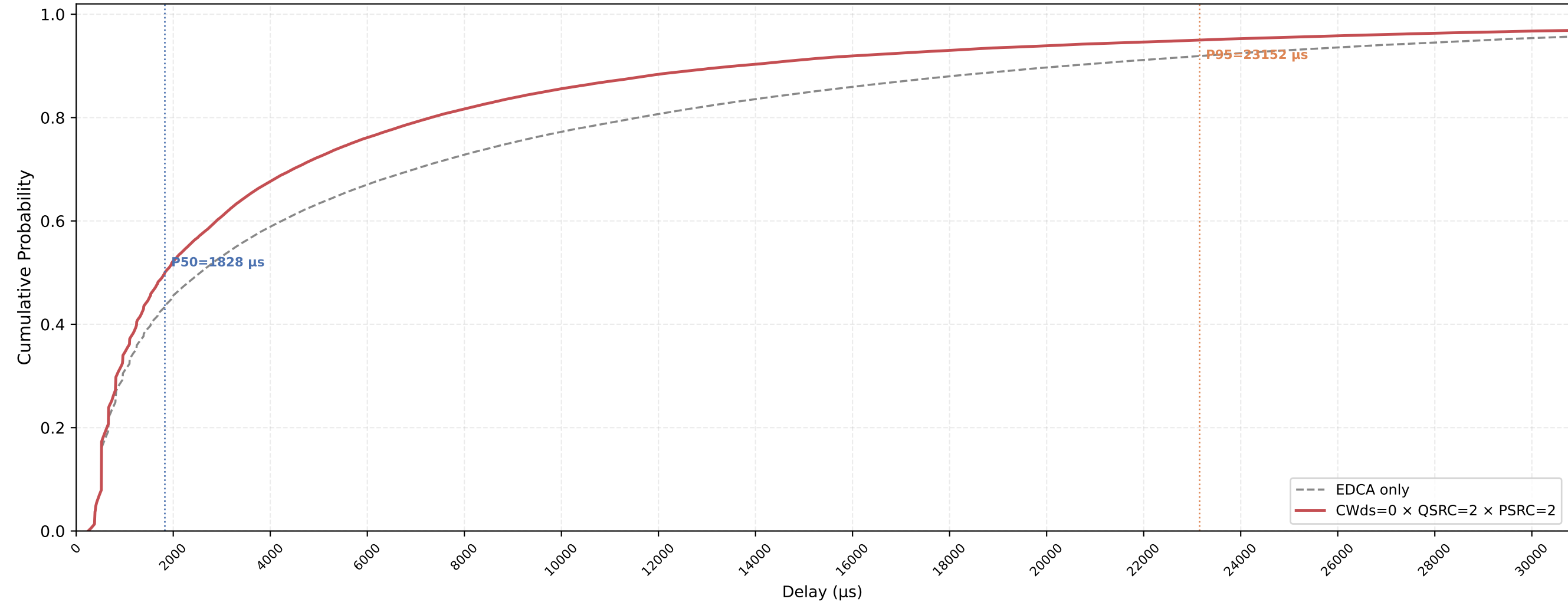
P-EDCA STA VO Delay CDF — CWds=0 × QSRC=2 × PSRC=2 nSta=30, nPedca=15, 1Mbps, avg of 10 runs
