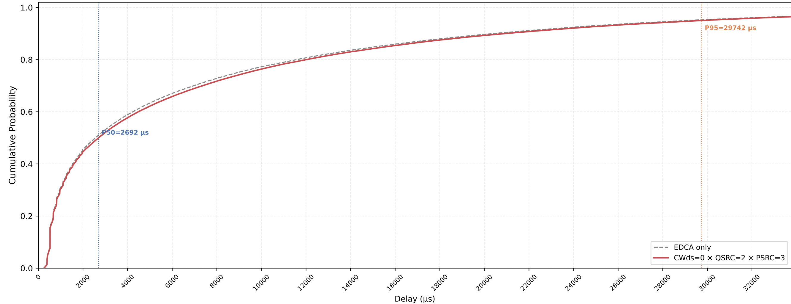
Legacy STA VO Delay CDF — CWds=0 × QSRC=2 × PSRC=3 nSta=30, nPedca=5, 1Mbps, avg of 10 runs
