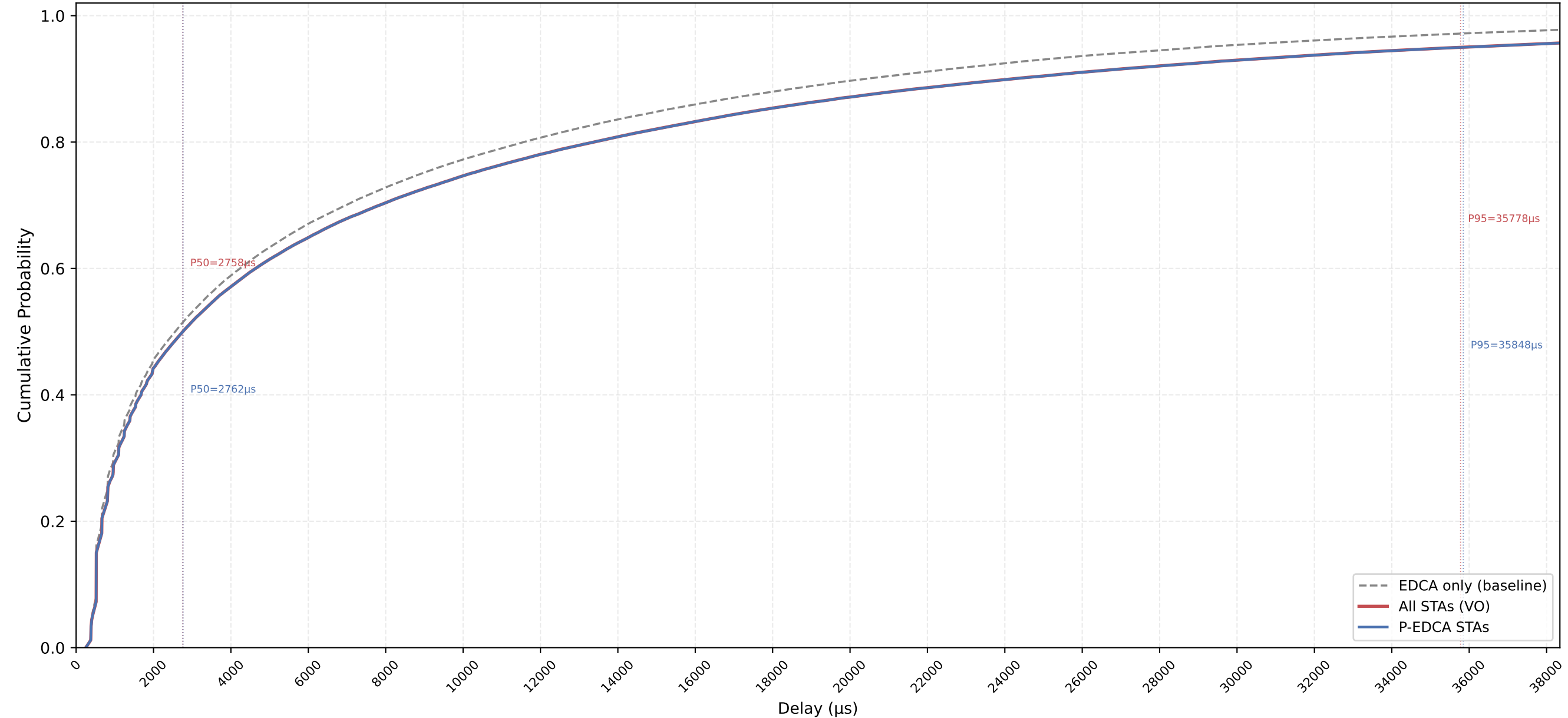
VO Delay CDF — P-EDCA / Legacy / All | CWds=0 × QSRC=5 × PSRC=3 nSta=30, nPedca=30/30, 1Mbps, avg of 10 runs
