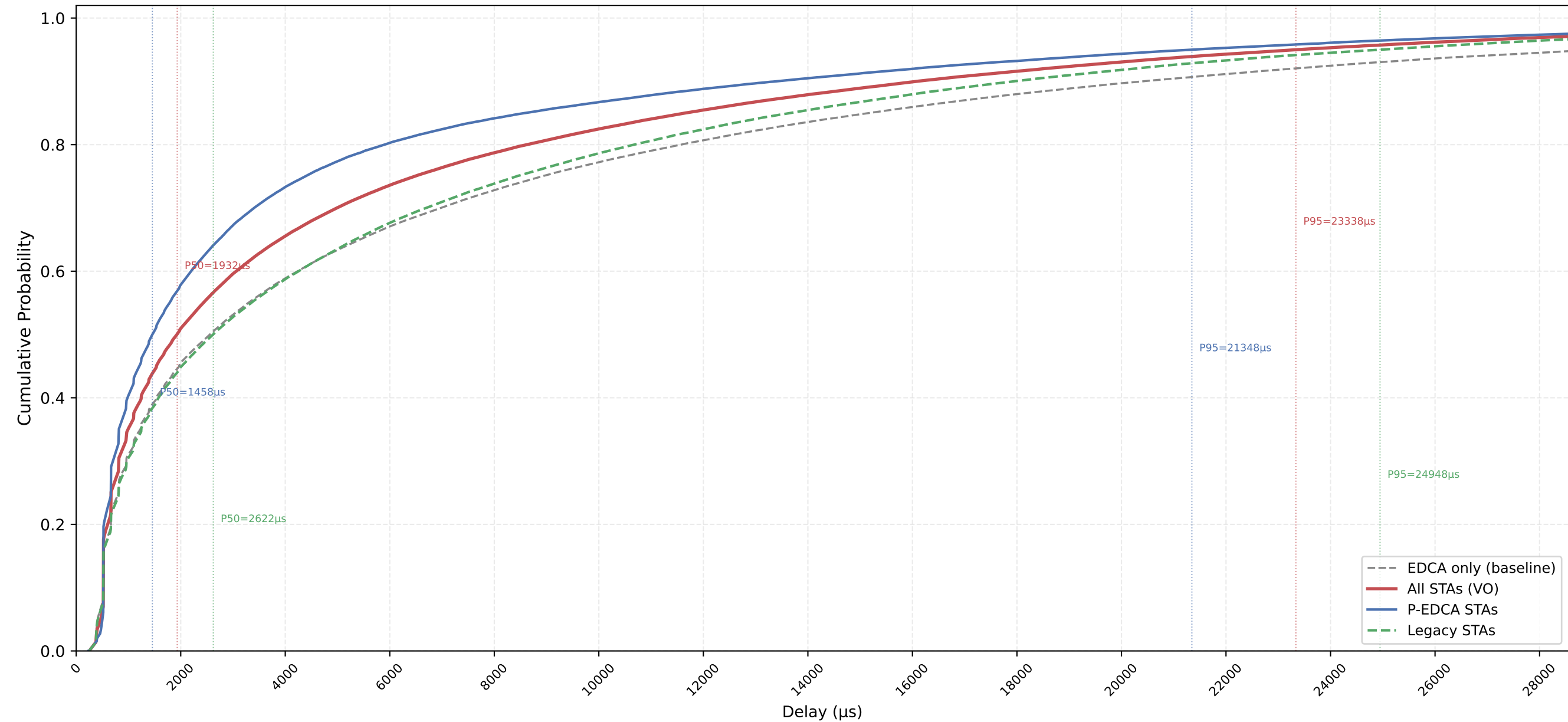
VO Delay CDF — P-EDCA / Legacy / All | CWds=1 × QSRC=0 × PSRC=1 nSta=30, nPedca=15/30, 1Mbps, avg of 10 runs
